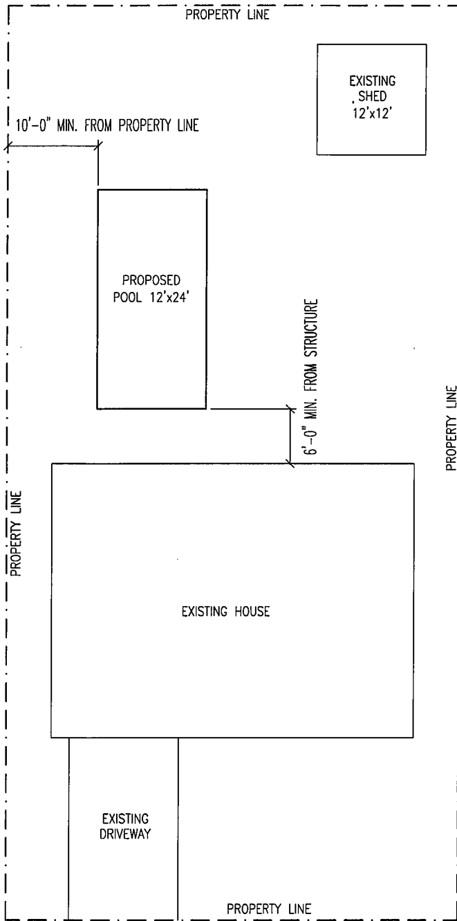
SITE PLAN SCALE: 3/32"=1'-0"
