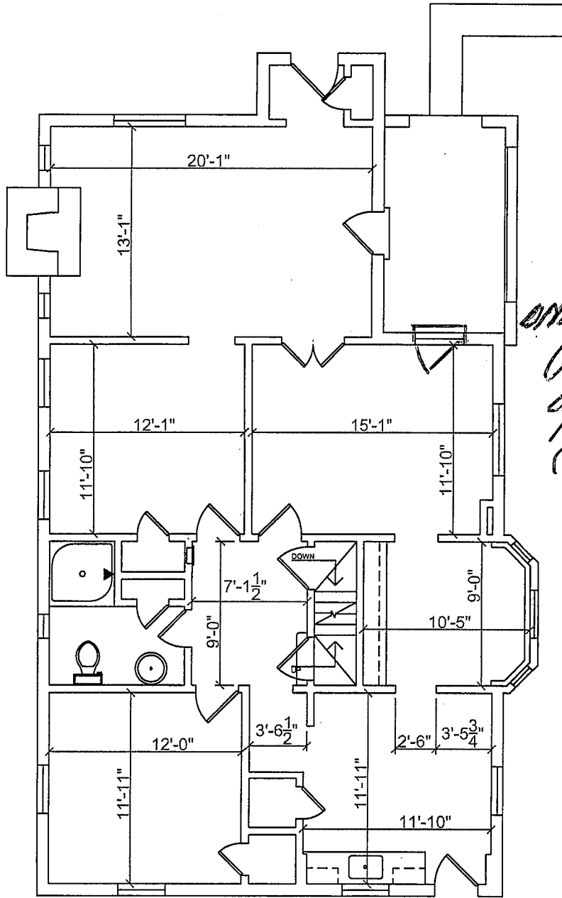
FIRST FLOOR
