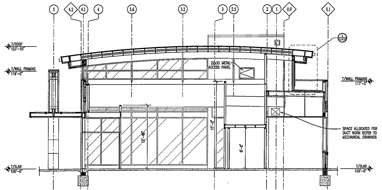
1 BUILDING SECTION SCALE: 3/16" = 1'-0"
