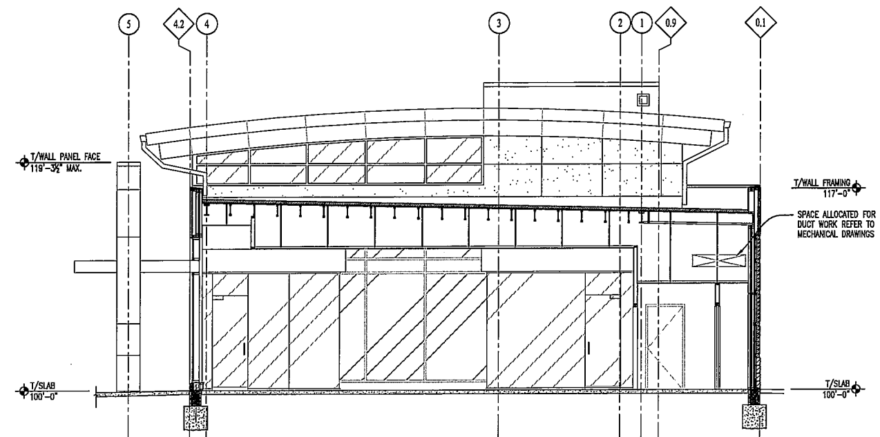
2 BUILDING SECTION SCALE: 3/16" = 1'-0"
