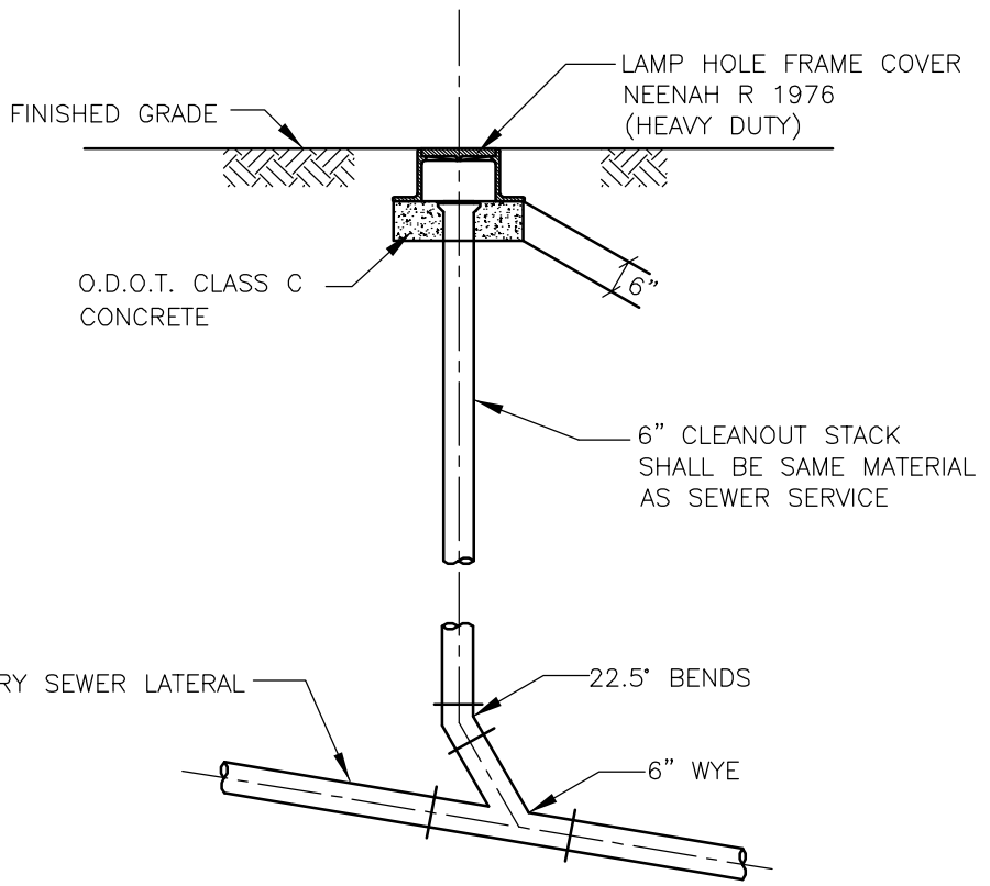
TYPICAL INLINE CLEAN OUT DETAIL
