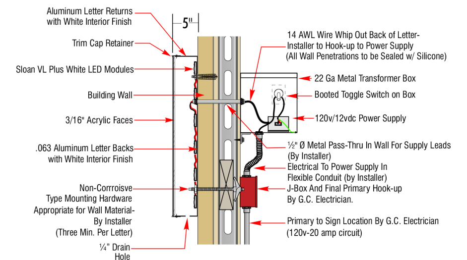
SECTION DETAIL - LED ILLUMINATED WALL LETTERS
