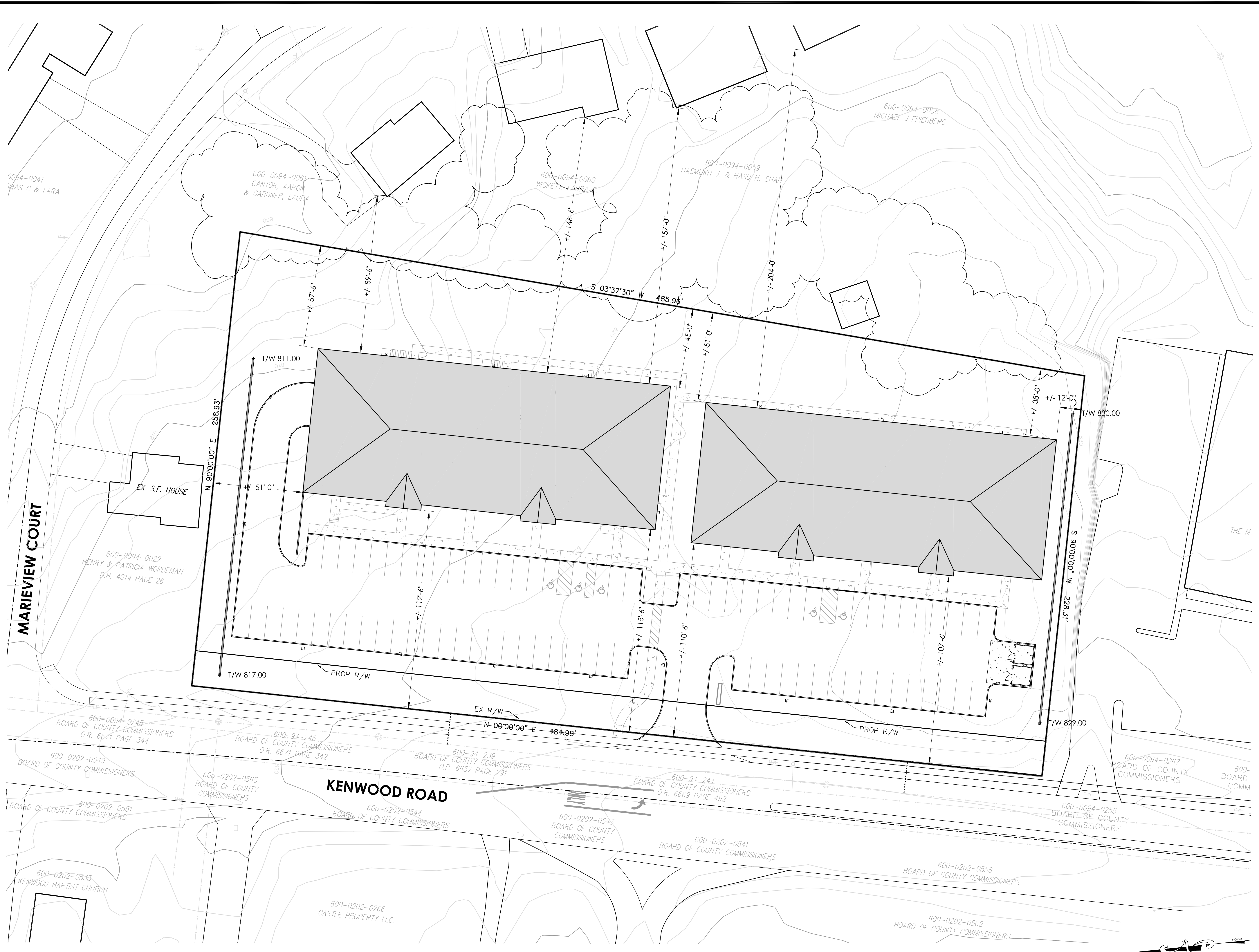
DIMENSION/SETBACK PLAN SCALE: 1"=30'
