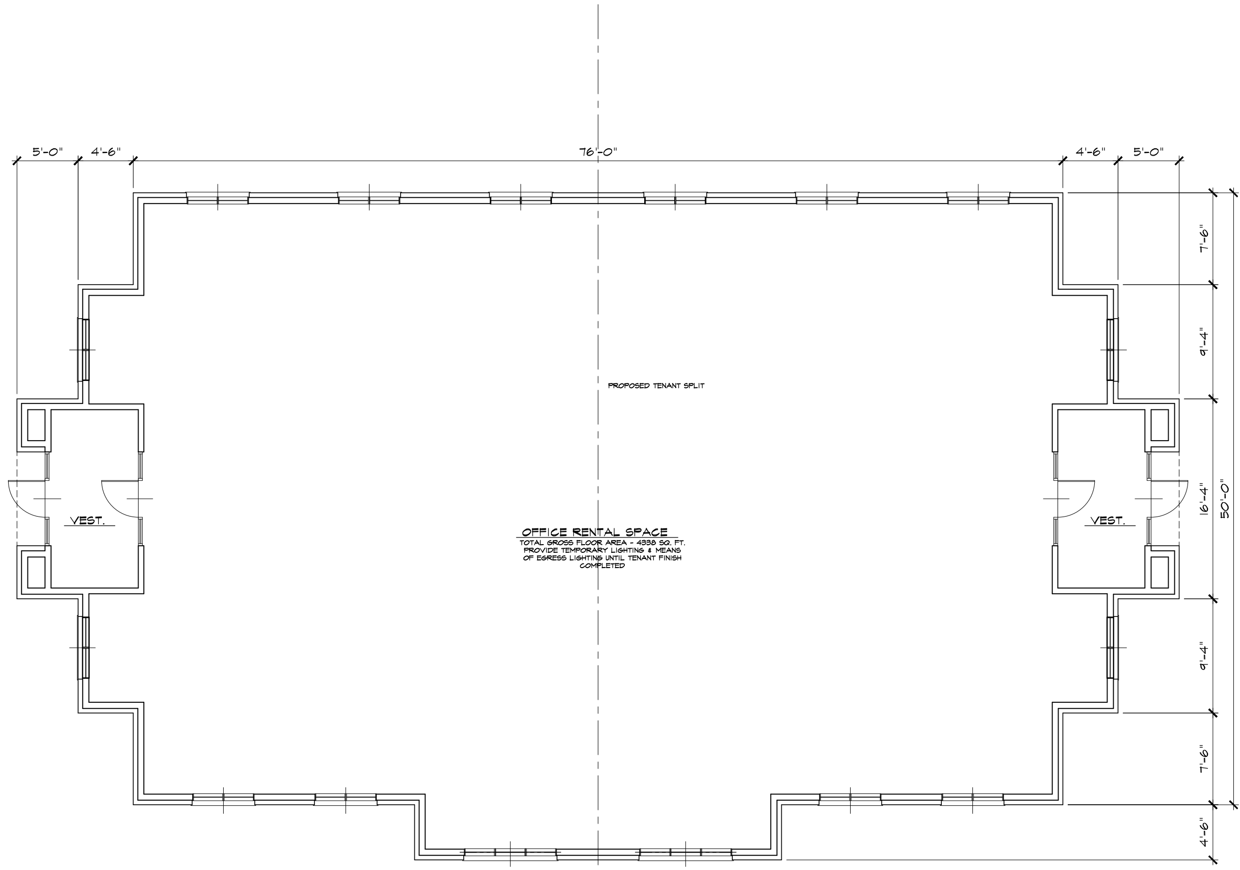
FLOOR PLAN 1/8"=1'-0" (1/A2)
