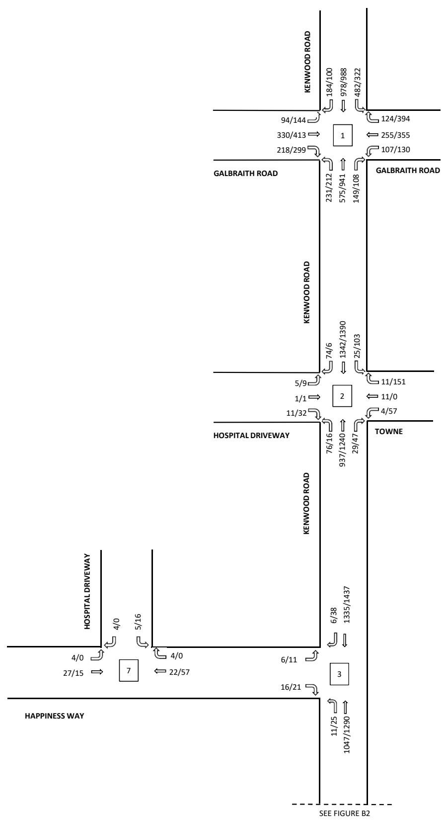
FIGURE B1 2018 EXISTING BLACK FRIDAY KENWOOD TIS, KENWOOD, OHIO XX/XX - MID/PM
