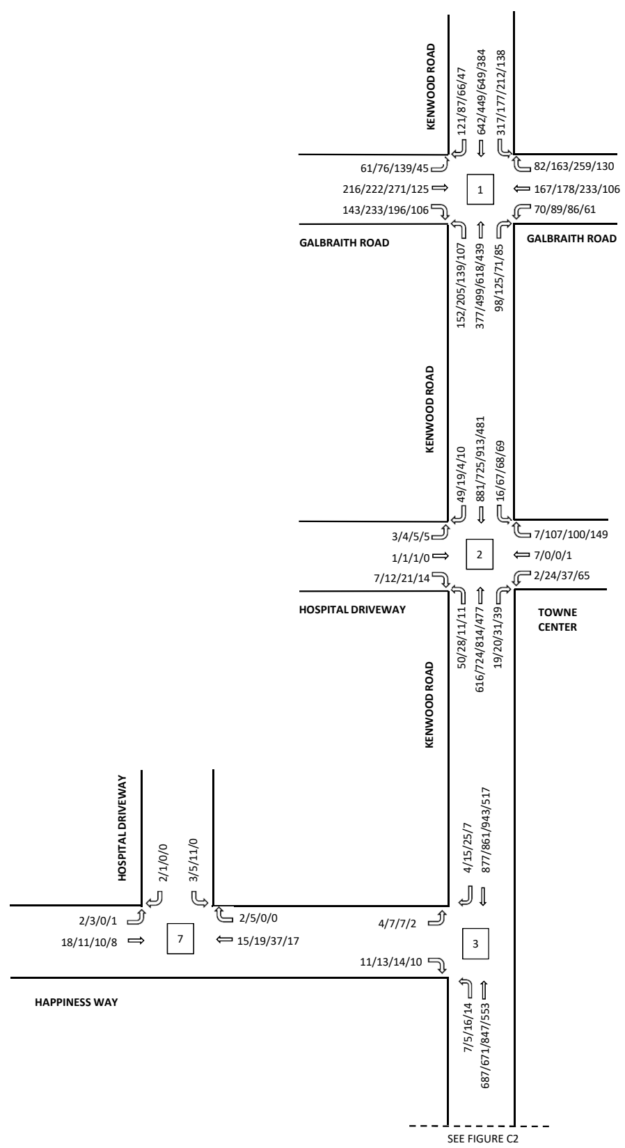
FIGURE C1 2020 BACKGROUND TRAFFIC KENWOOD TIS, KENWOOD, OHIO XX/XX/XX/XX - AM/Midday/PM/SAT
