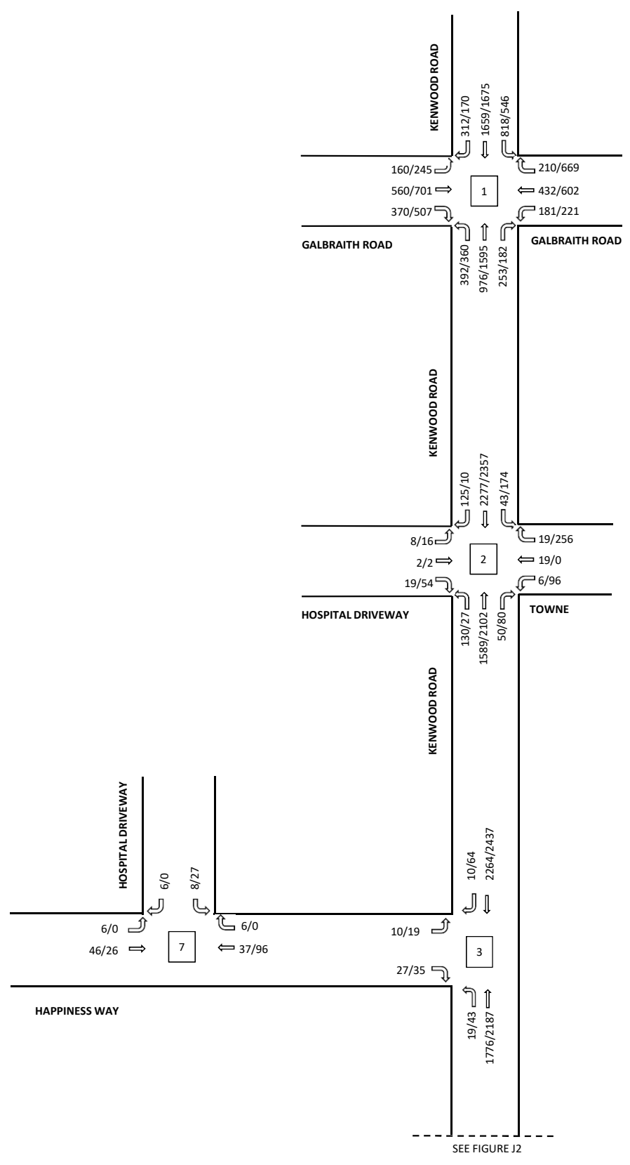
FIGURE J1 2040 BACKGROUND BLACK FRIDAY KENWOOD TIS, KENWOOD, OHIO XX/XX - MID/PM
