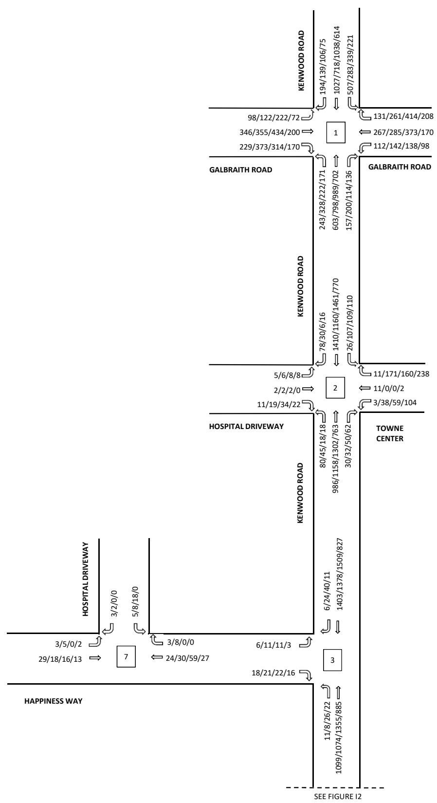
FIGURE I1 2040 BACKGROUND TRAFFIC KENWOOD TIS, KENWOOD, OHIO XX/XX/XX/XX - AM/Midday/PM/SAT
