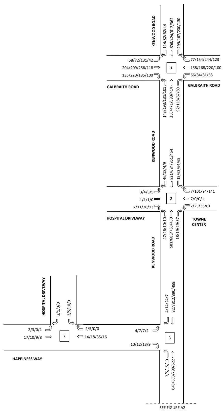
FIGURE A1 2018 EXISTING TRAFFIC KENWOOD TIS, KENWOOD, OHIO XX/XX/XX/XX - AM/Midday/PM/SAT
